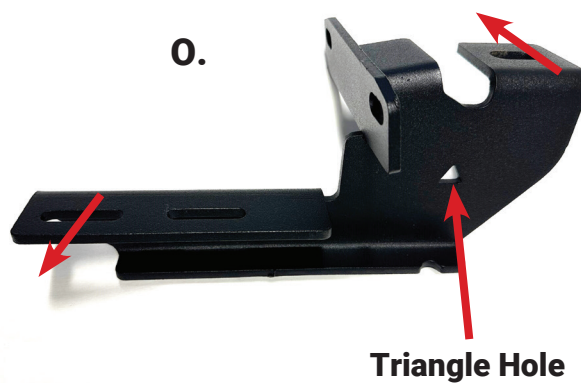
Left Rear Mounting Bracket
