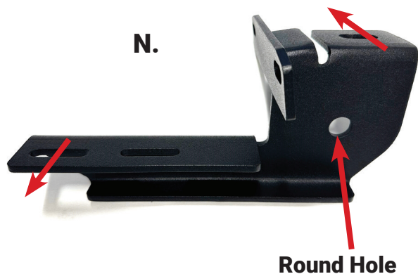
Left Front Mounting Bracket
